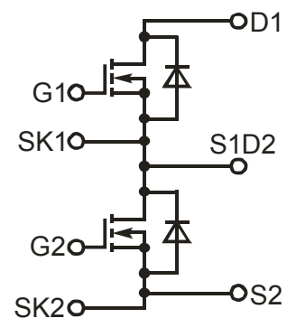
Figure 2 – Electric circuit of internal module's connections
