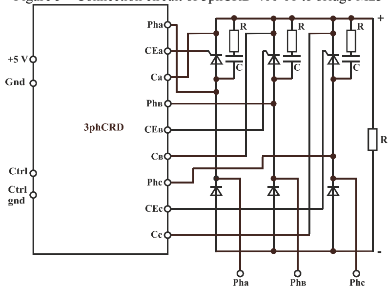
Figure 6 – Connection circuit of 3phCRD-400-01 to diode-thyristor modules
