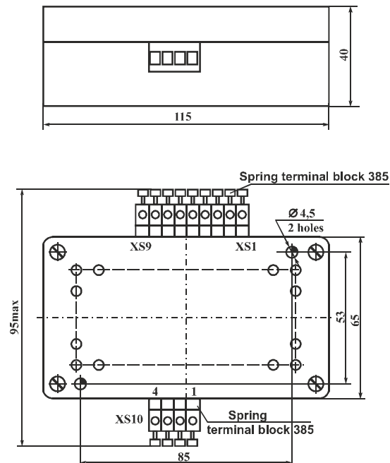
Figure 3 – Overall drawing of 3phCRD-400-01
