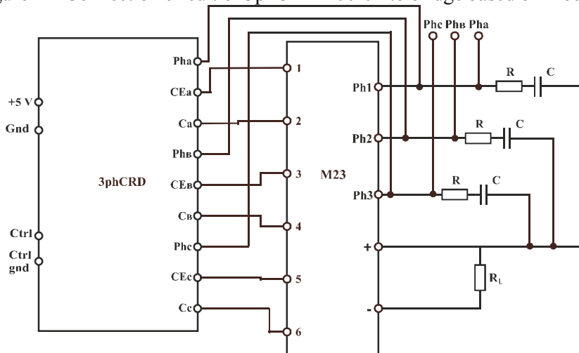
Figure 5 – Connection circuit of 3phCRD-400-01 to bridge M23
