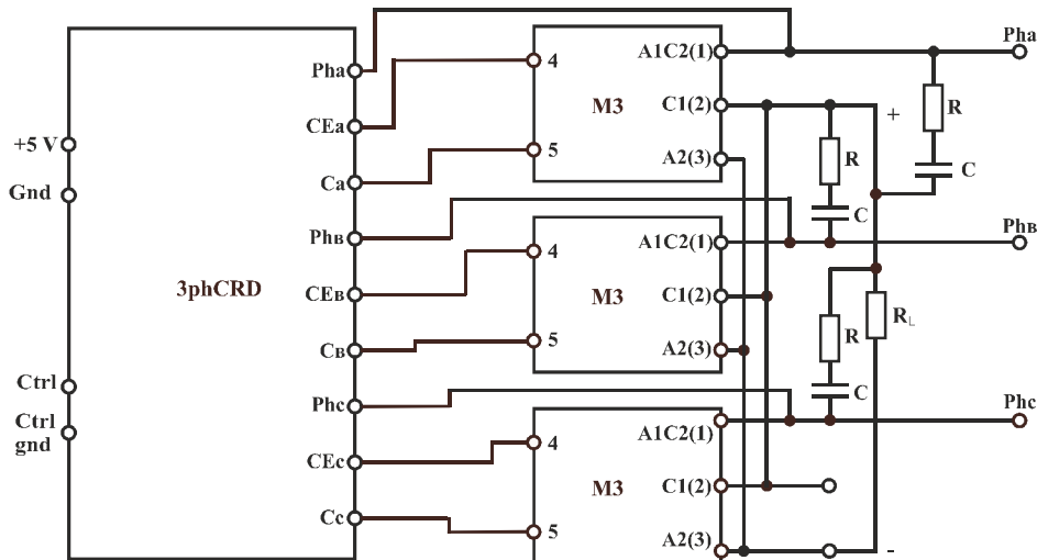
Figure 4 – Connection circuit of 3phCRD-400-01 to bridge based on modules M3
