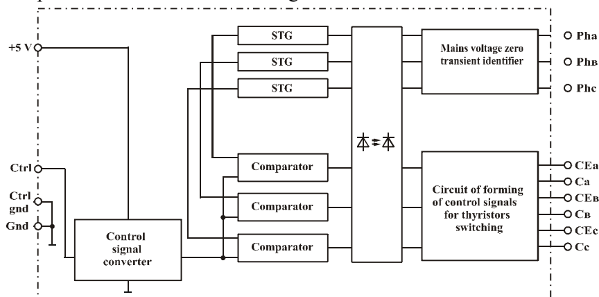
Figure 1 – Functional circuit of 3phCRD-400-01
